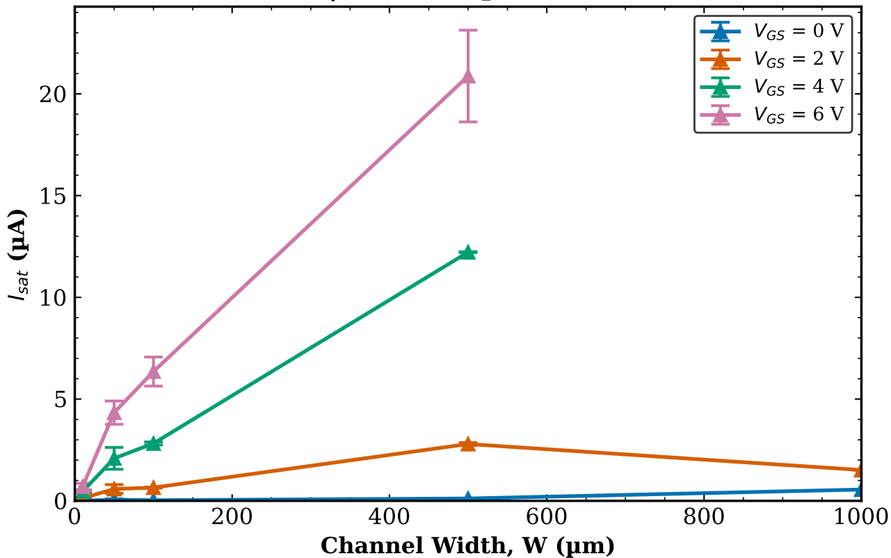
TFT2 Combined (Tr. 1 & 2) I_{sat} vs W | L = 160\text{ }\mu\text{m} (mean \pm std)
